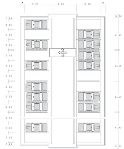
Parkebene parking level
